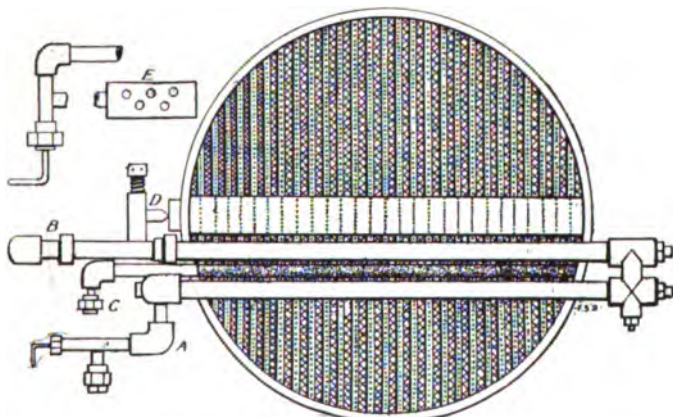
FIG. 215.—The Tubulous Gasoline Burner of the Lane Carriage. A is the tube leading from the gasoline tank and across the burner space; B, the tube leading from the vaporizer tubes to the pilot burner, main feed and regulator; C, the tube for pouring alcohol into the torch; D, the connection of the main burner feed and nozzle; E, elevation of B, showing pilot burner.
